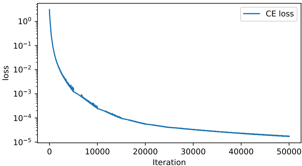
Cross Entropy loss with 4 layer Transformer pos off on tiny_extract_m404 H=1.6156
